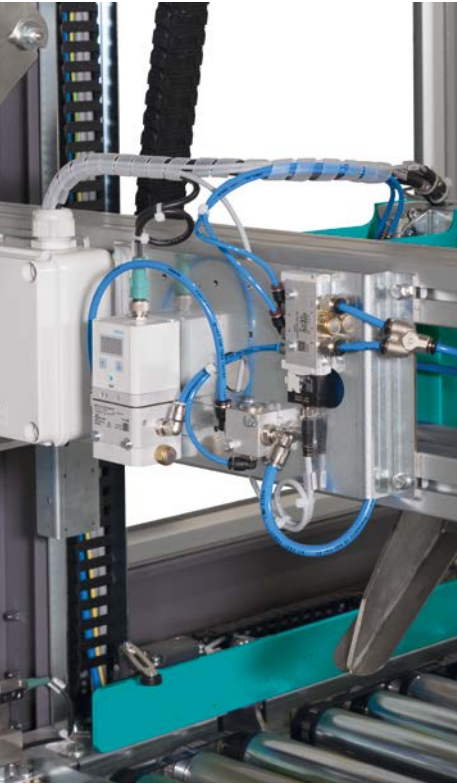
Fig. 3 DCM - inside
